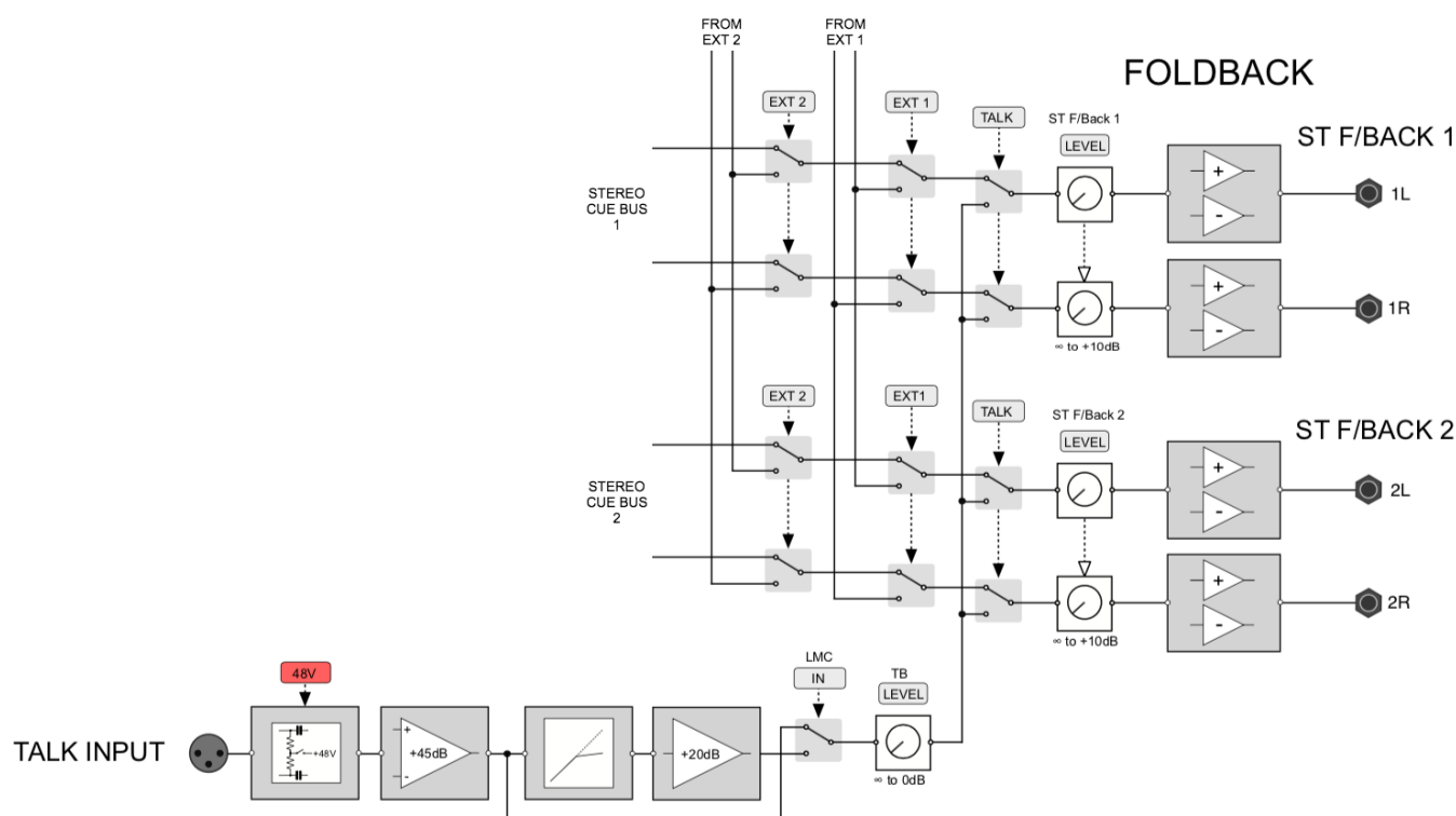
SiX Foldback Block Diagram
